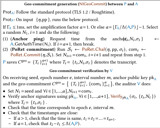
Figure 8: Geo-commitment protocols.
